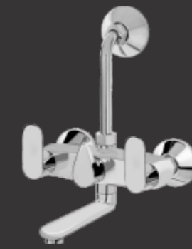
O-017 Wall Mixer Telephonic With 'L' Bend for ARR. Of O/H Shower
